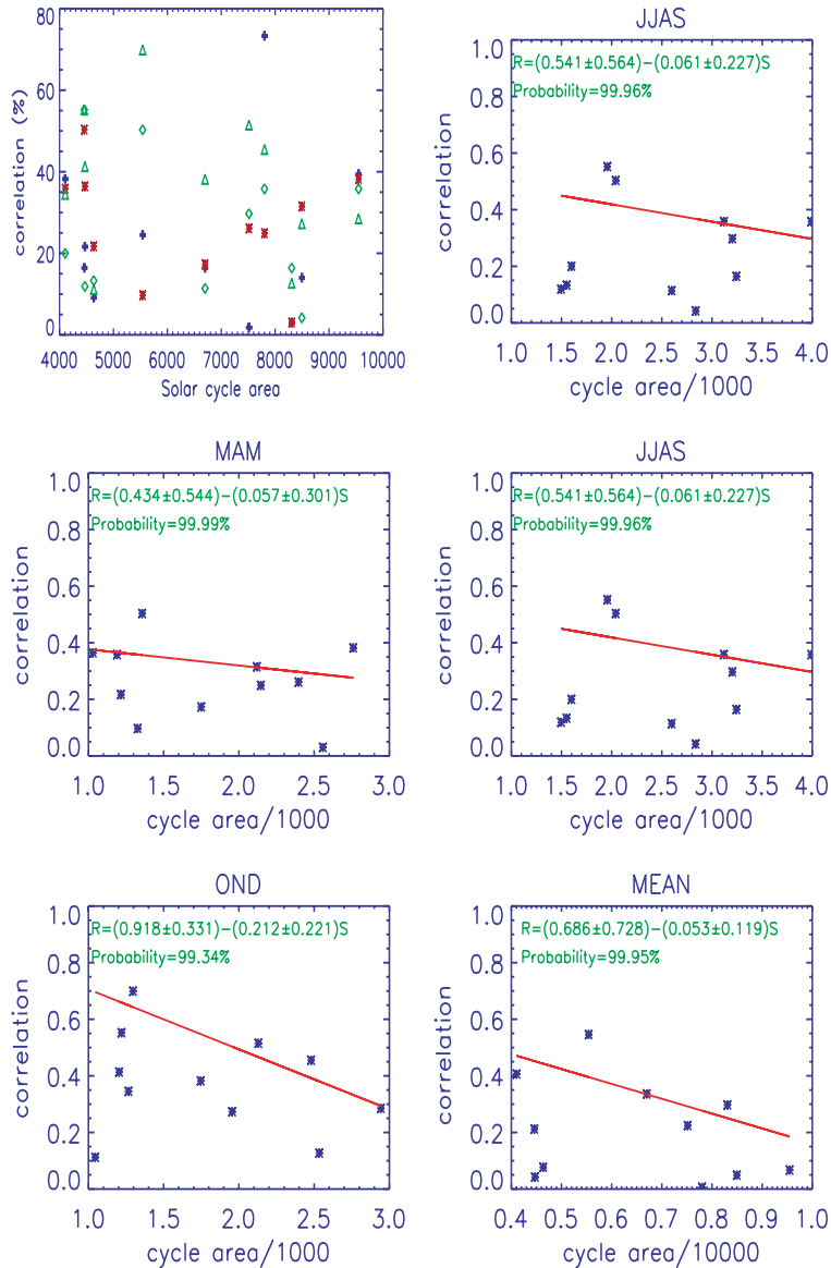
Figure 1. Different cycle-to-cycle variations of the correlation coefficients for the seasonal months are plotted against the annual area of the solar cycle. Different symbols in the first plot are: JF as +, MAM as *, JIAS as ◇ and OND as △. The rest of the plots represent the same as in the first plot, except that data are presented separately (for different seasonal months) with a line (in red colour) that is obtained from the linear least square fit is also over plotted.
